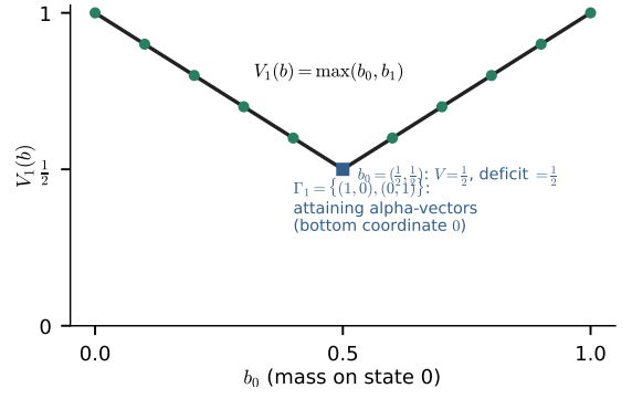
Figure 5: The two-floor chance instance: the one-step value is \max(b_0, b_1) , attained by the alpha-vectors of \Gamma_1^\Pi = \{(1,0), (0,1)\} with zero bottom coordinate (green probes); at the symmetric prior the value is \frac{1}{2} and the deficit equals the minimal mass.
